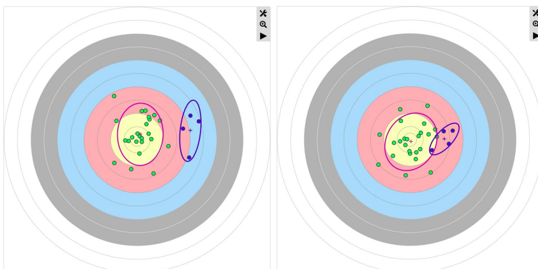
Figure 14: Bare Shaft Test for Arrow Length
